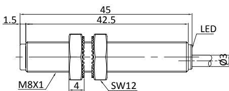
Fig. 1 Inductive sensor with cable (flush)
